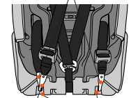
Top Tether Tether/LATCH Storage
